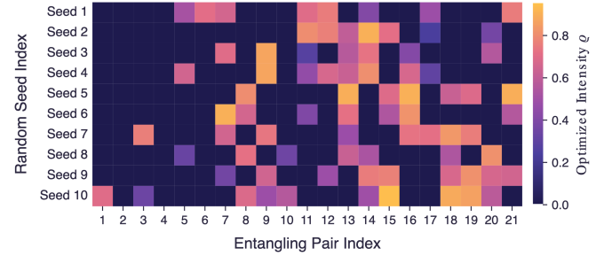
FIG. 8 Family-of-wells sparsity: final pair intensities \kappa(p) = \sum_P r_{P,P} for 10 random seeds (rows) across the 21 LPTE entangling pairs (columns). Dark cells are pruned parameters ( \rho < 0.05 ); each seed retains a different sparse subset.
