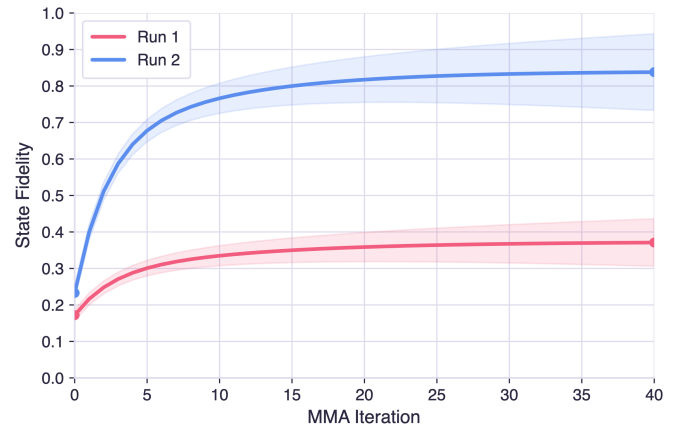
FIG. 3 Two representative 8-qubit LPTE trajectories under triple-channel correlated noise (Run 1: 0.172 \rightarrow 0.371 ; Run 2: 0.233 \rightarrow 0.838 ). Shaded bands are \pm 1 standard deviation across the 10-seed ensemble.
